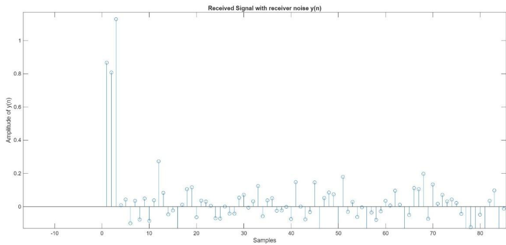
Figure 3: Zoom In Channel Sounding Output
