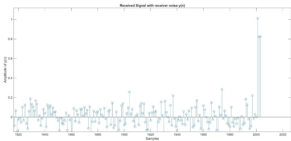
Figure 4: Zoom In Channel Sounding Output
